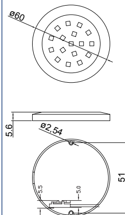
Fixture dimensions
